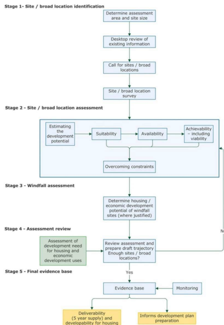
Figure 2.1 Land Availability Assessment Methodology Flowchart (Extract from Planning Practice Guidance)
